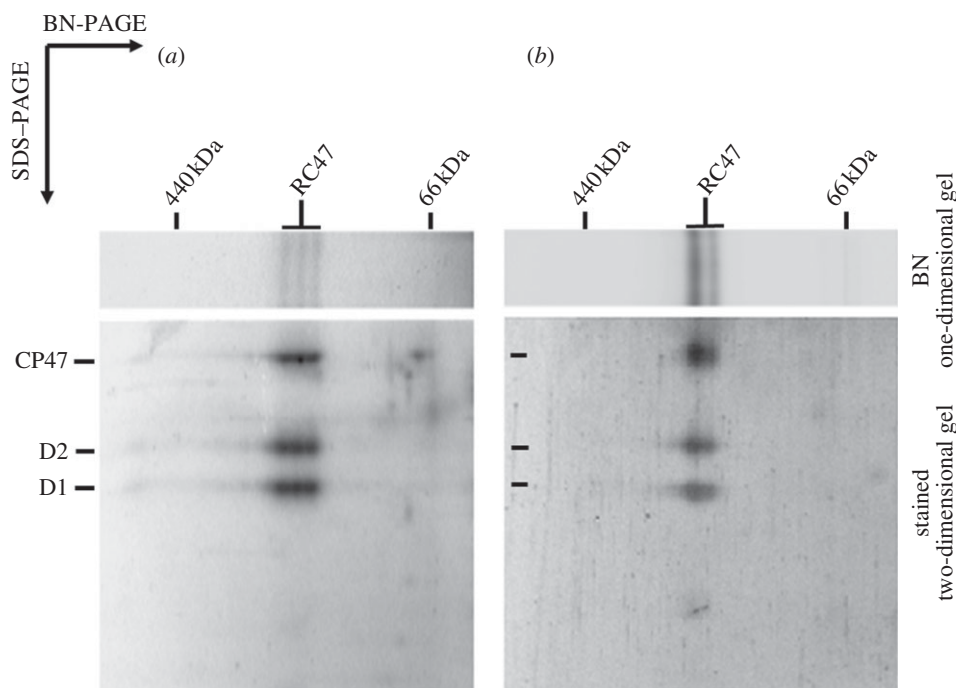
Figure 2. Two-dimensional analysis of RC47 complexes isolated from thylakoid membranes of Synechocystis strains expressing (a) His-tagged Psb28 or (b) FLAG-tagged Psb28-2. Complexes corresponding to an amount of 1 \mu\text{g} Chl a were separated on a 4–14% (w/v) polyacrylamide (PAA) CN–PAGE linear gradient gel, and another 12–20% (w/v) PAA SDS–PAGE gel was used for the second dimension. The gels were stained with Sypro Orange. The position of the monomeric RC47 is indicated.
