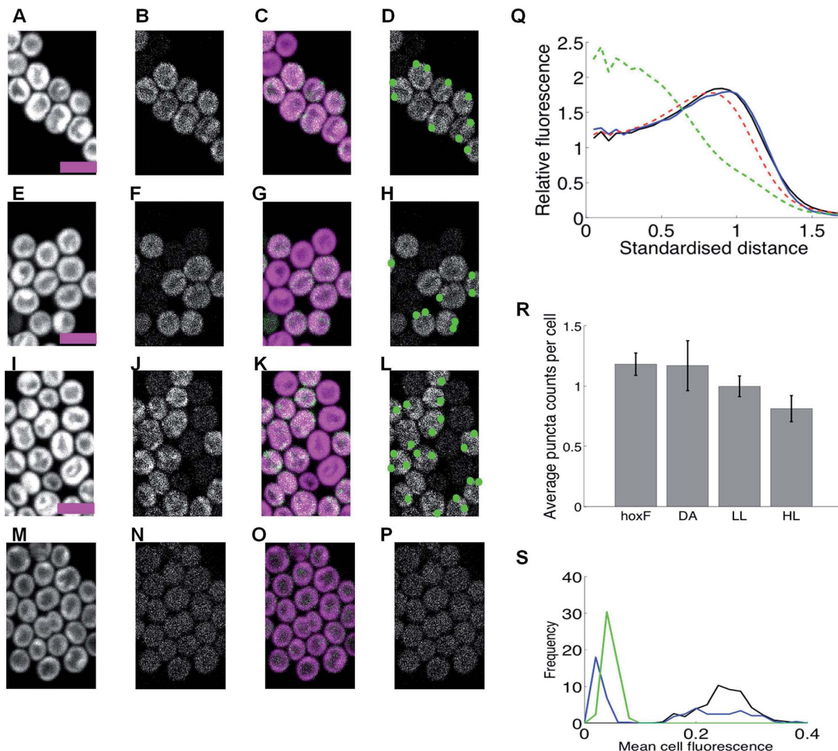
Fig. 4 HoxF-GFP distribution and patterning in M55 (Complex I-deficient) and \Delta hoxHY mutants grown in low light, high light, under dark adaptation and anoxia (no oxygen). (A–D) M55 under low light (LL). (E–H) M55 after 10 min high light exposure (HL). (I–L) M55 after 5 days dark adaptation (DA). (M–P) \Delta hoxHY under low light (LL). Columns in (A–P) as Fig. 1. Scale-bars 5 microns. (Q) Radial distribution of fluorescence: free GFP (green); chlorophyll (red) HoxF-GFP (black); HoxF-GFP in M55 background (expressing cells, blue). Standardised distance refers to rescaling the 1/2 maximum radius for chlorophyll to a radial distance of 1. (R) Mean counts of HoxF-GFP puncta/cell in M55 background under DA, HL, LL and anoxia with SEM over replicate experiments (6, 2, 2, and 2 respectively). DA HoxF-gfp cells repeated from Fig. 1R, (S) Mean HoxF-GFP fluorescence per cell under LL for HoxF-GFP (black), M55 background (blue) and \Delta hoxHY background (green). Fluorescence is corrected for cell autofluorescence by subtracting cell fluorescence after photobleaching. Data in Q–R from 291–492 cells by condition.
